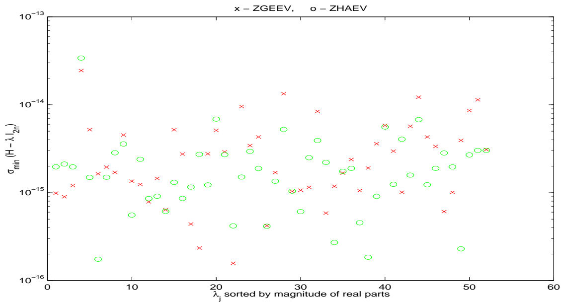
Figure 1: Example 4, backward error of computed eigenvalues ( n = 50 ).
